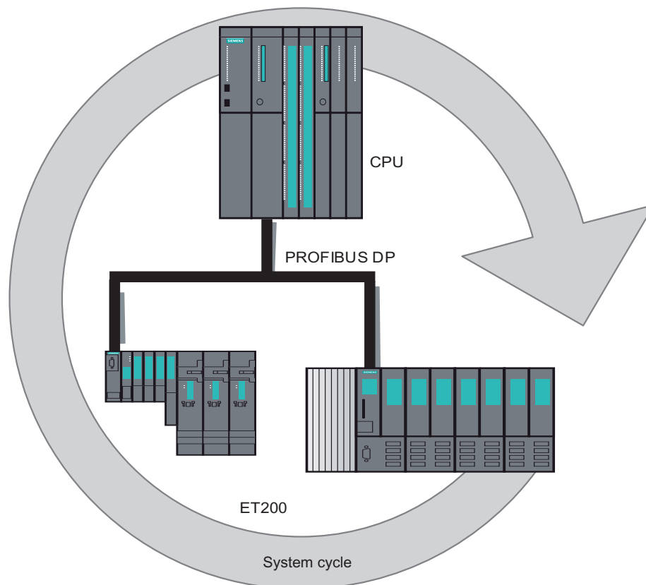
Figure 5-9 Just-In-Time
