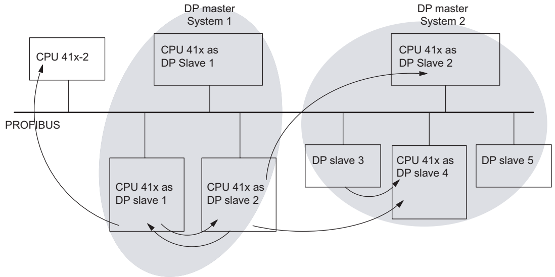
Figure 5-7 Direct data exchange with 41x CPUs
