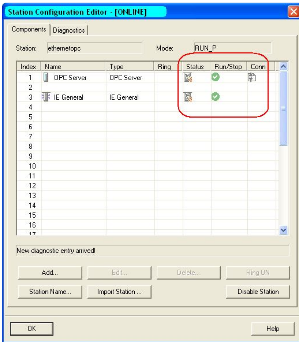
图 22: PC Station 运行状态
