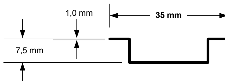
Fig. 6. Dimensions for installation on a top-hat rail
