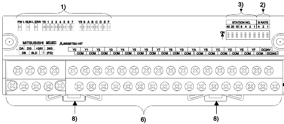
AJ65SBTB3-8 □ (8点端子排模块, 3线)
