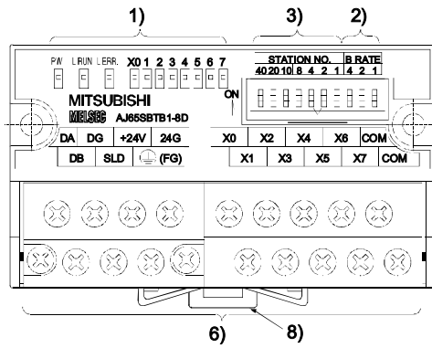
AJ65SBTB1-16 □ (16 点端子排模块, 单线)
