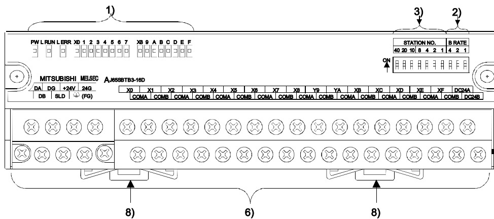
AJ65SBTB3-16 □ (16点端子排模块, 3线)
