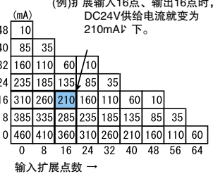
FX2N-48ER-UA1/UL
