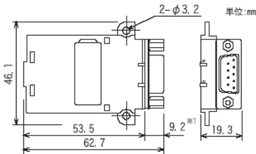
FX3U-422-BD
