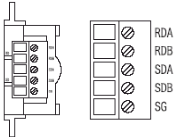
FX3U-485-BD
