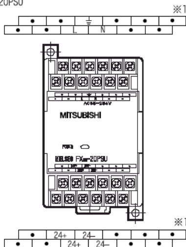
FX2N-20PSU
