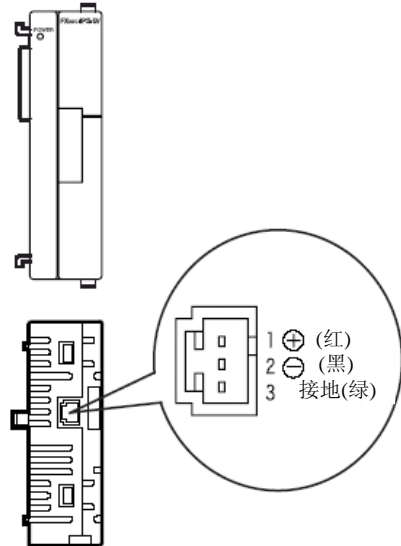
FX3UC-1PS-5V
