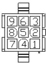
HOUSING: AMP (1-172161-9)
