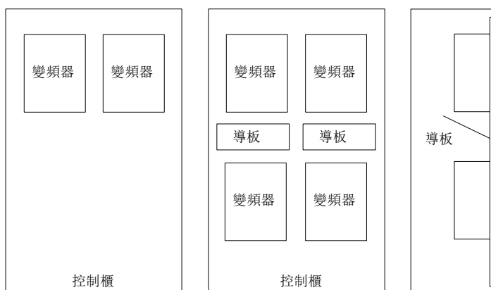
(a)橫向排列
