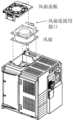
FR-E740-3.7K-CHT的示例
