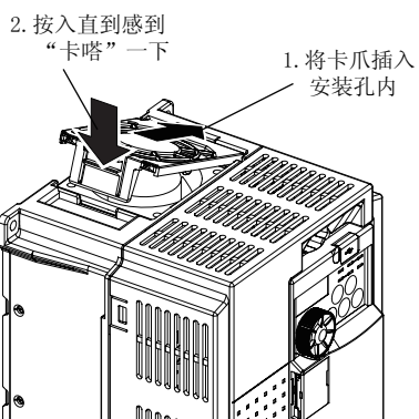
FR-E740-3.7K-CHT的示例
