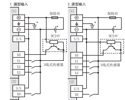
[1]:CPU模块, FX5-32E□ [2]:输入模块
