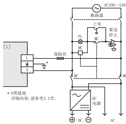
[1]:CPU模块, FX5-32E□
