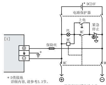
[1]:CPU模块, FX5-32E□
