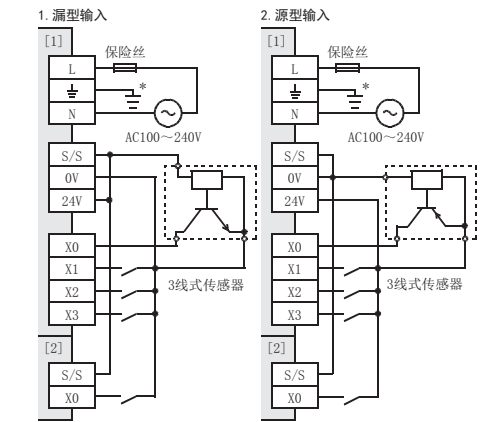
[1]:CPU模块, FX5-32E□ [2]:输入模块
