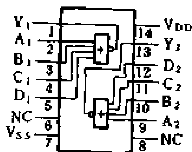
CC4002 双 4 输入或非门 Y = \overline{A + B + C + D}
