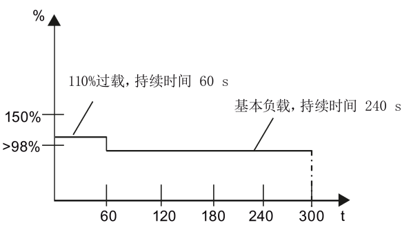
低过载模式允许的过载 (LO)
