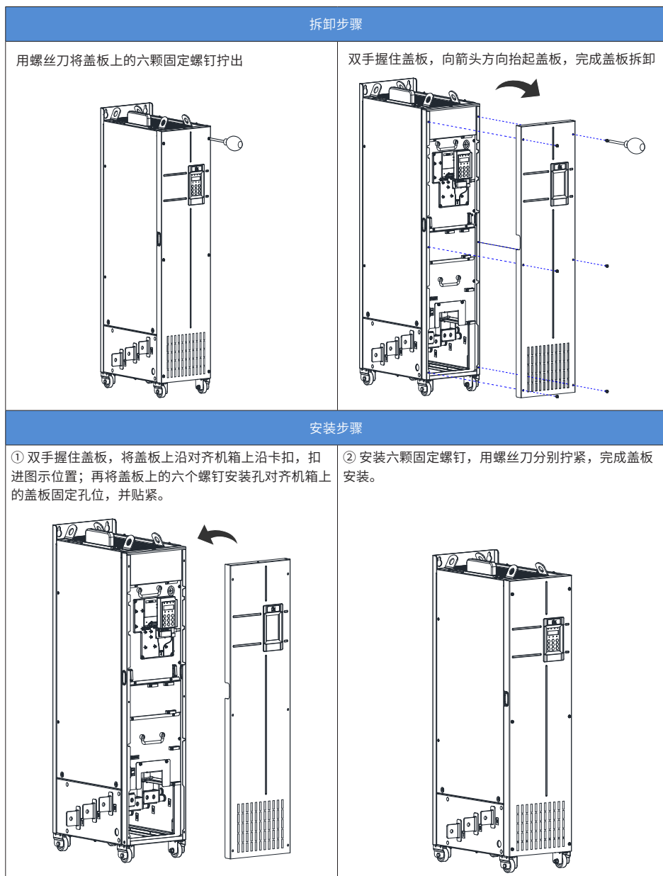
图 3-26 CP300T200G/220P~CP300T450G/500P 机型盖板拆卸与安装
