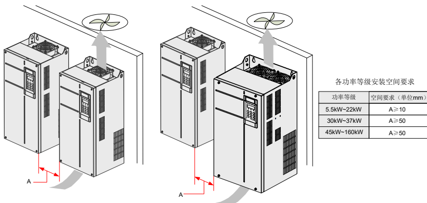
图 3-4 CP300T5.5G/22P~CP300T160G/ 机型多台机器并排安装
