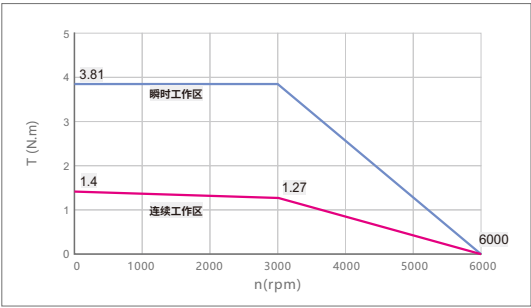
SMC60S-0040-30□K-5LSU
