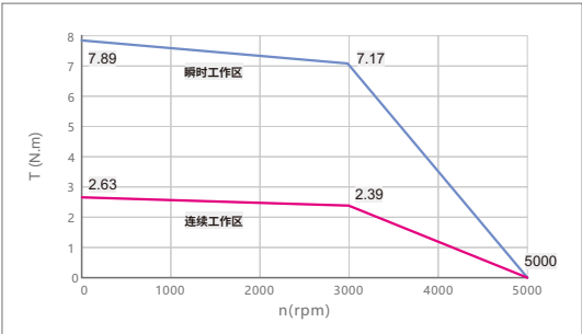
SMC80S-0075-30□□K-5LSU
