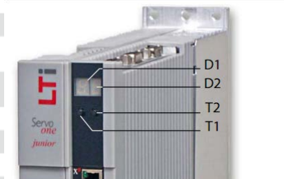
Figure 4.1 Integrated operator control unit
