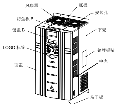
W02 (塑壳)
