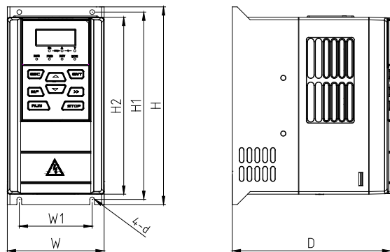
a) EV1S-08G/15L-EV1S-37G/55L
