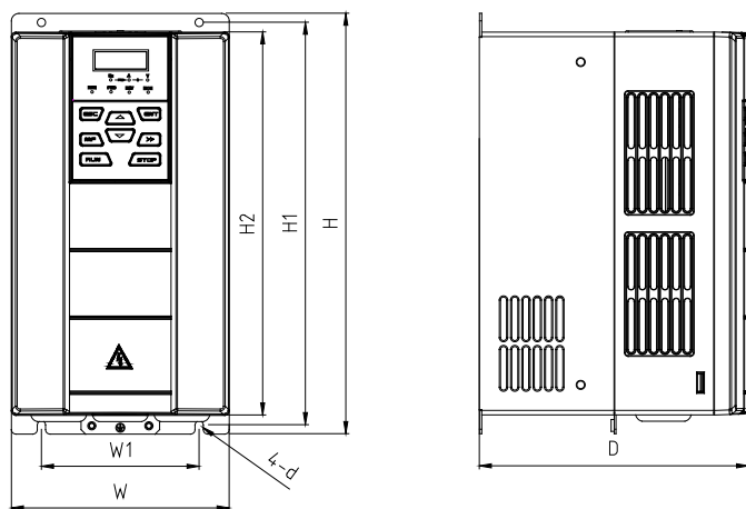
b) EV1S-55G/75L-EV1S-2BG/3ZL
