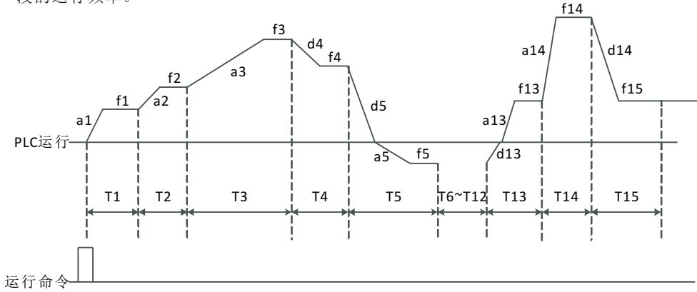
图5-33 PLC单循环后保持终值
