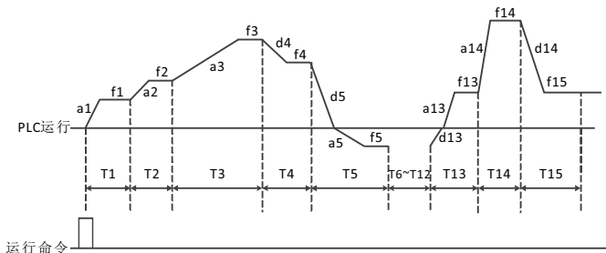
图5-33 PLC单循环后保持终值
