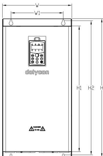
b) 适用于 CT100-4T-15G/18.5P ~ CT100-4T-110G/132P
