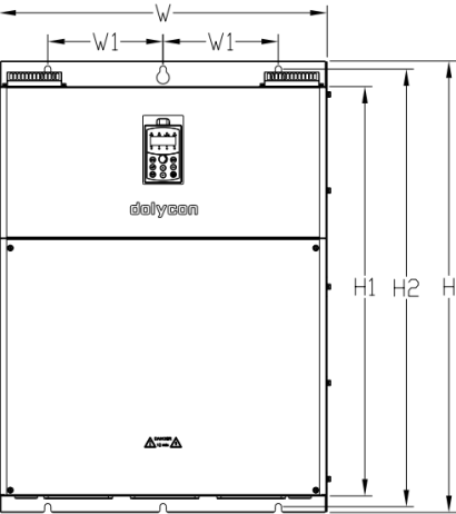
d) 适用于 CT100-4T-220G/250P ~ CT100-4T-315G/350P
