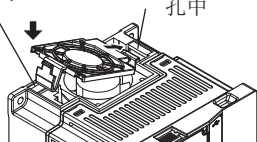
FR-F820-00105 (2.2K) ~ FR-F820-00250 (5.5K) FR-F840-00083 (3.7K)、 FR-F840-00126 (5.5K)
