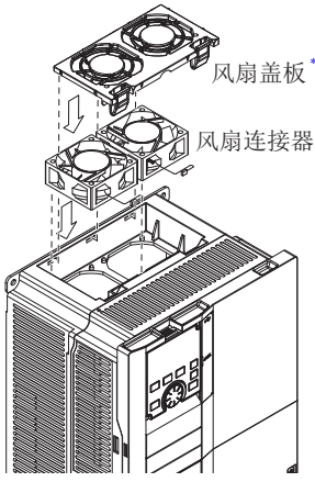
FR-F820-00340 (7.5K) ～ FR-F820-01540 (37K) FR-F840-00170 (7.5K) ～ FR-F840-00770 (37K)
