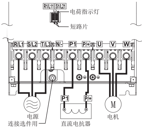
FR-F820-03800 (90K)、FR-F820-04750 (110K) FR-F840-03250 (132K) ~ FR-F840-04810 (220K)
