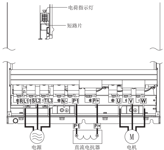
FR-F840-05470 (250K) ~ FR-F840-06830 (315K)
