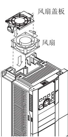
FR-F820-00105 (2.2K) ～ FR-F820-00250 (5.5K) FR-F840-00083 (3.7K)、 FR-F840-00126 (5.5K)
