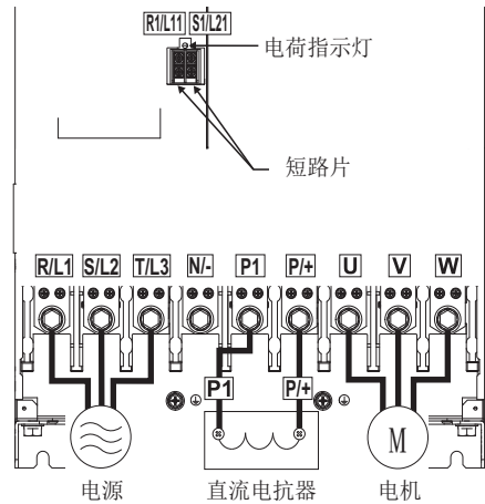
FR-F840-00930 (45K) ~ FR-F840-01800 (75K) *2
