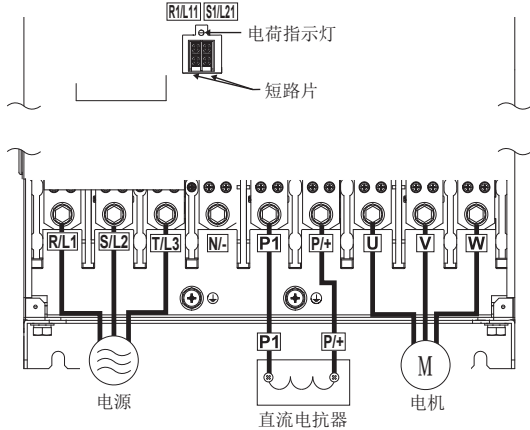
FR-F840-02160 (90K)、FR-F840-02600 (110K)
