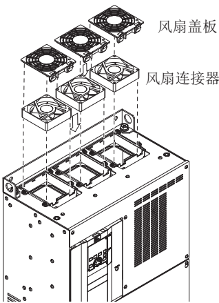
FR-F820-01870 (45K) 及以上 FR-F840-00930 (45K) ～ FR-F840-03610 (160K)
