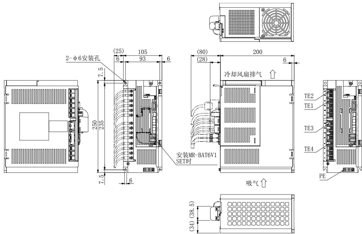
(f) MR-J4-500B(-RJ)
