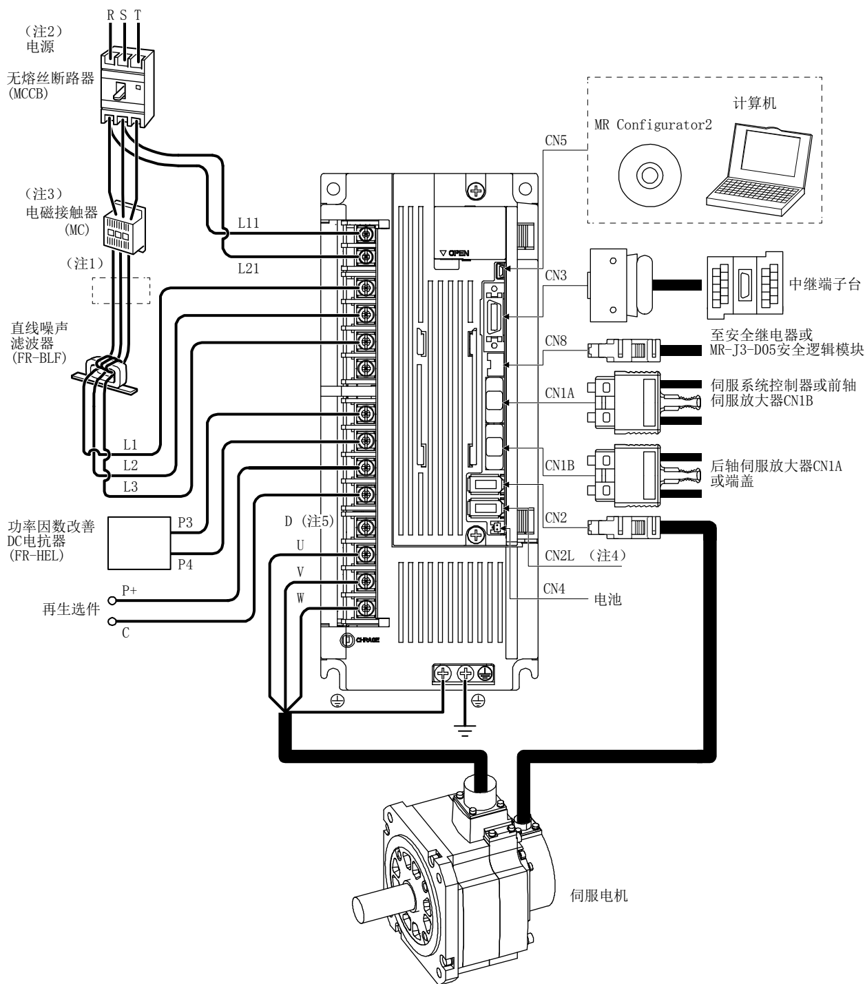
(c) MR-J4-500B (-RJ)
