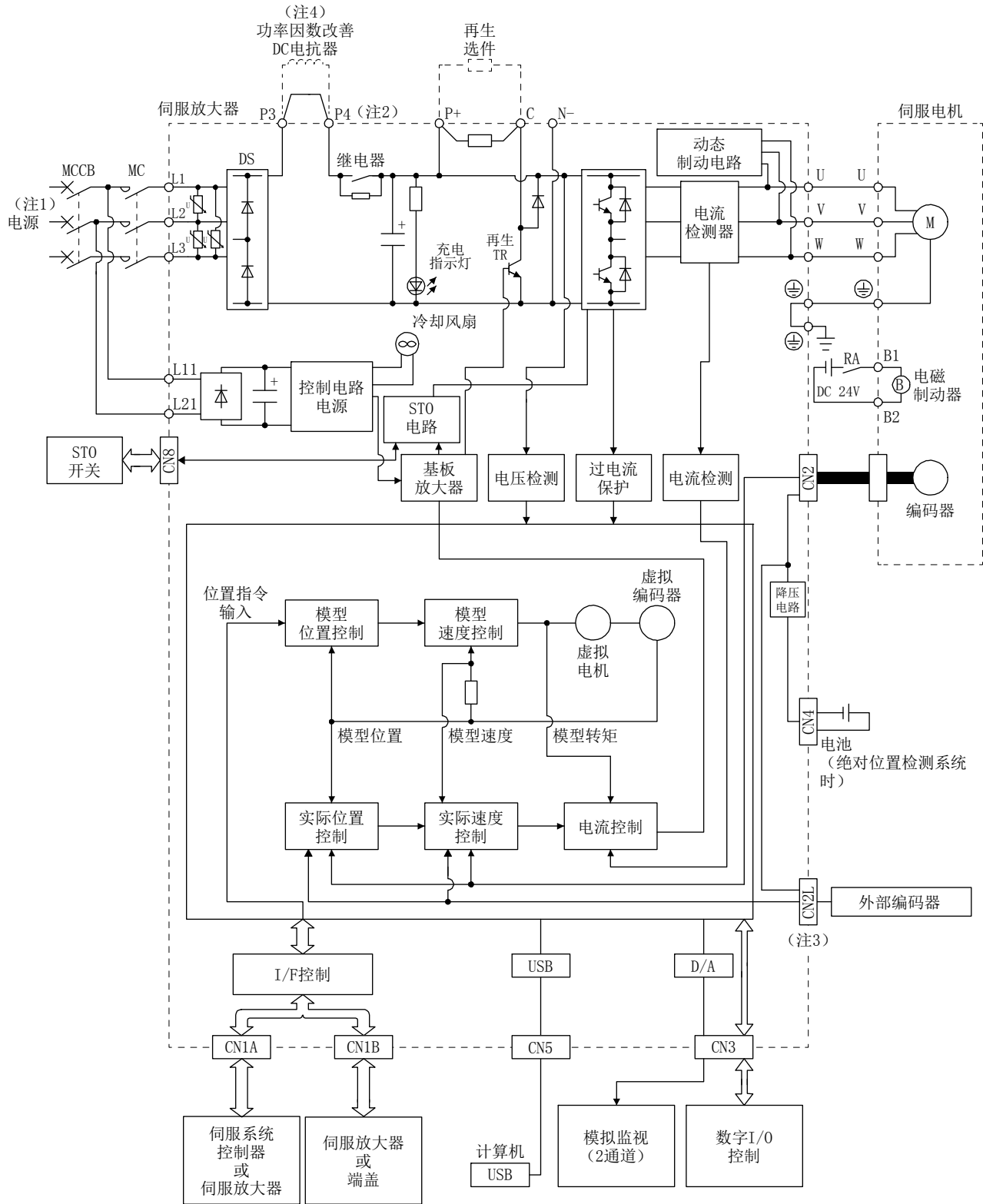
(b) MR-J4-700B(-RJ)
