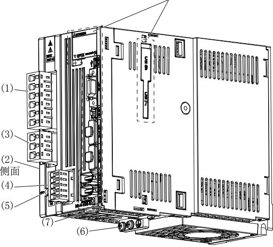
(b) MR-J4-350B(-RJ)
