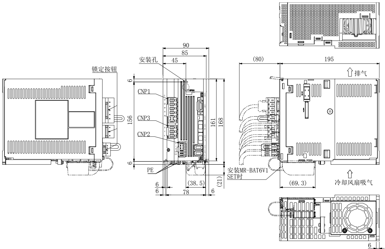
(e) MR-J4-350B (-RJ)
